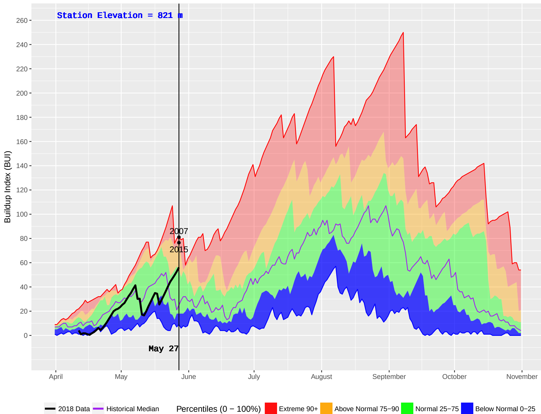
AKOKLI CREEK (838) : Historical (2003–2016) and Current (2018) Noon Buildup Index (BUI)
